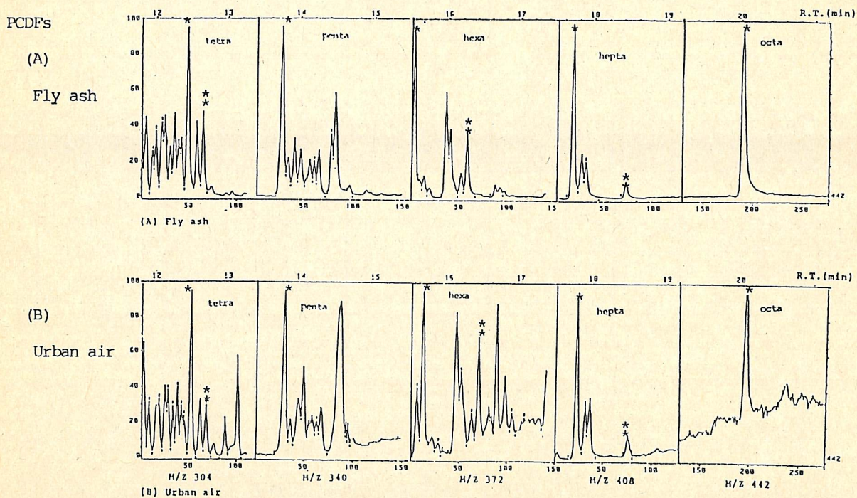
Fig. 3 GC-MS-SIM chromatograms of PCDFs.
