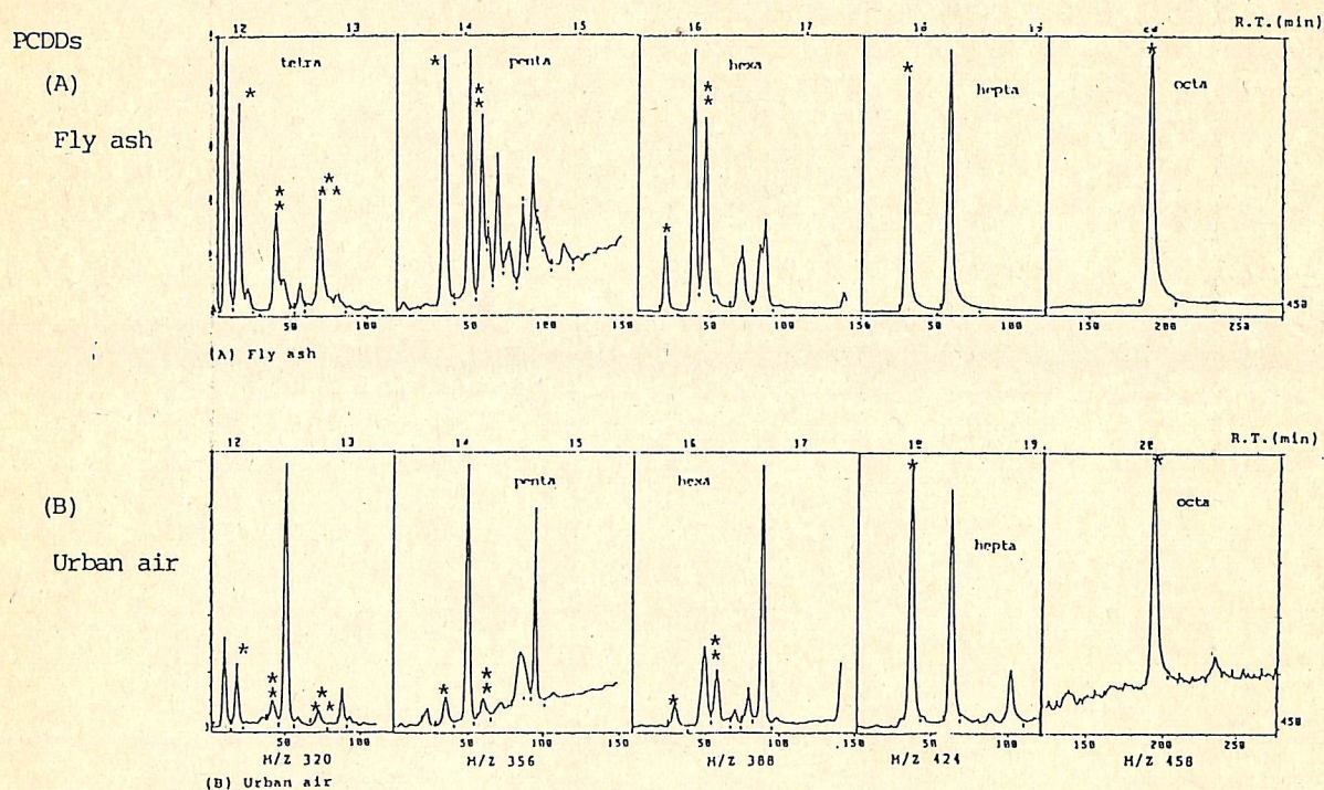
Fig. 2 GC-MS-SIM chromatograms of PCDDs.
