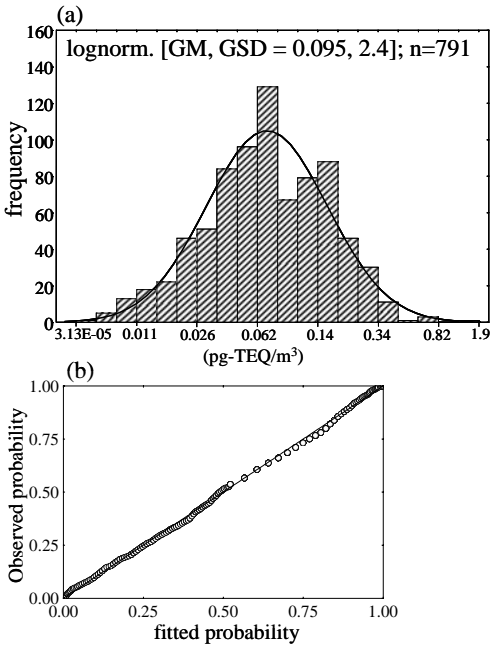
Figure 2: (a)Histogram and curve fitting of dioxin concentration in air (fiscal 2001). X-axis is in natural logarithmic scale. Data from the vicinity of pollution sources were excluded. (b) the P-P plots of air.
