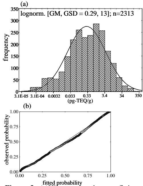
Figure 3: (a)Histogram and curve fitting of dioxins concentration in soil (fiscal 2001). X-axis is in natural logarithmic scale. Data from the vicinity of pollution sources were excluded. (b) the P-P plots of soil.
