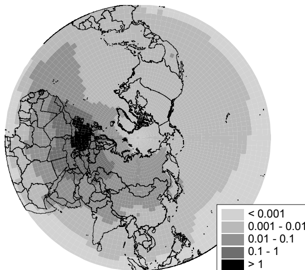
Figure 4.1 Spatial Distribution of Mean Annual \gamma -HCH Concentrations in the Surface Air Over the Northern Hemisphere for 1990, \text{ng}/\text{m}^3 (Malanichev, 2002)
